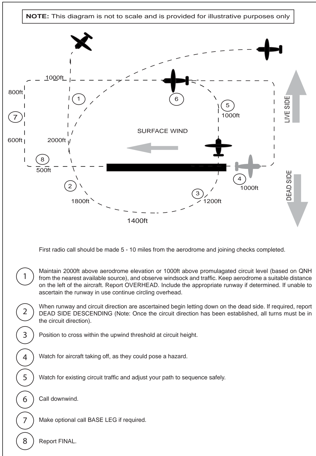
Figure 2 Standard Overhead Join Procedure See paragraph 1.8.3 for additional information regarding overhead join procedures
