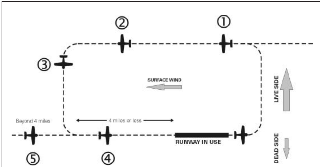
Figure 1 Designated positions in the traffic circuit Typical Left-Hand Circuit
