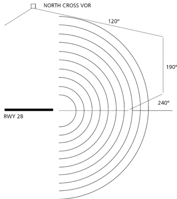
Figure 1 Radar vectors to an ILS approach
